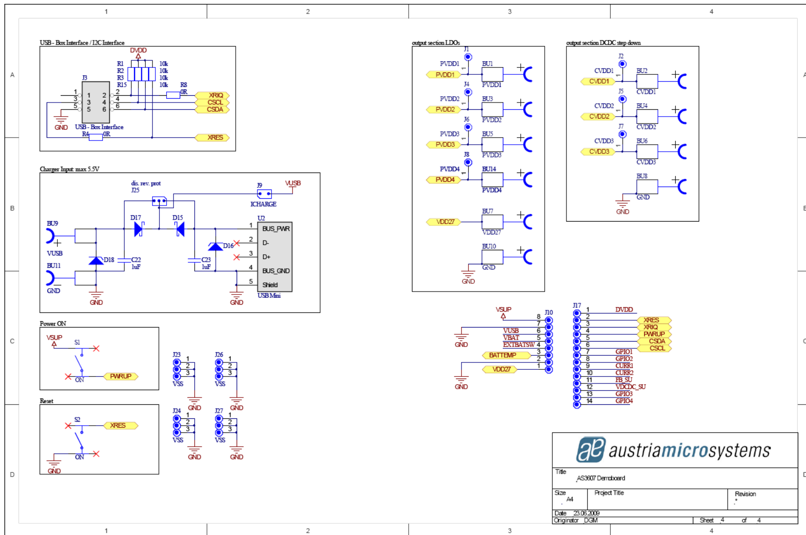
Application Schematic AS3607 Evalboard 1v0 – page2
