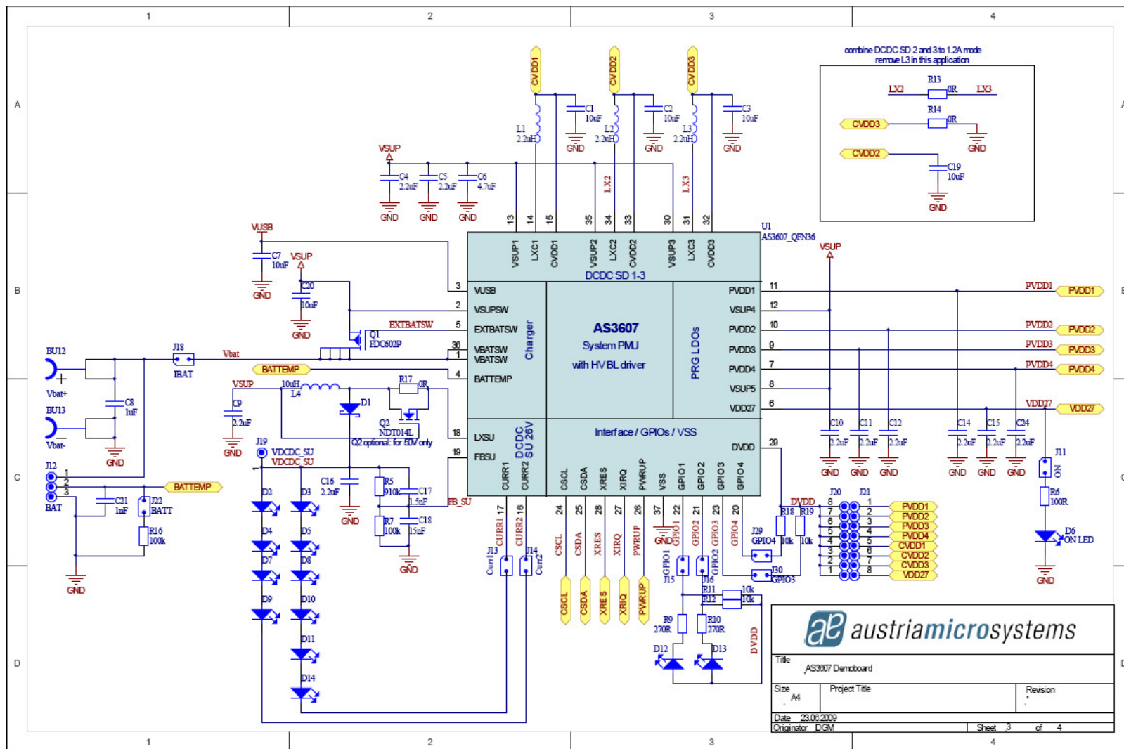
Application Schematic AS3607 Evalboard 1v0- page 1
