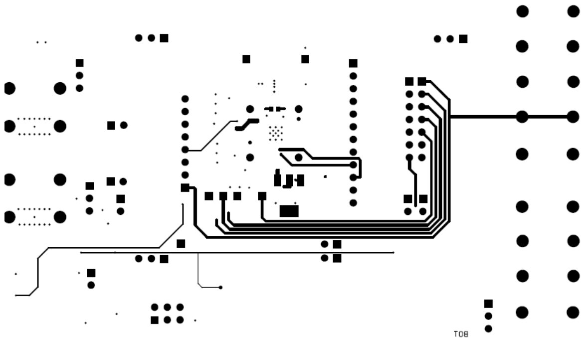
Layout (bottom view)
