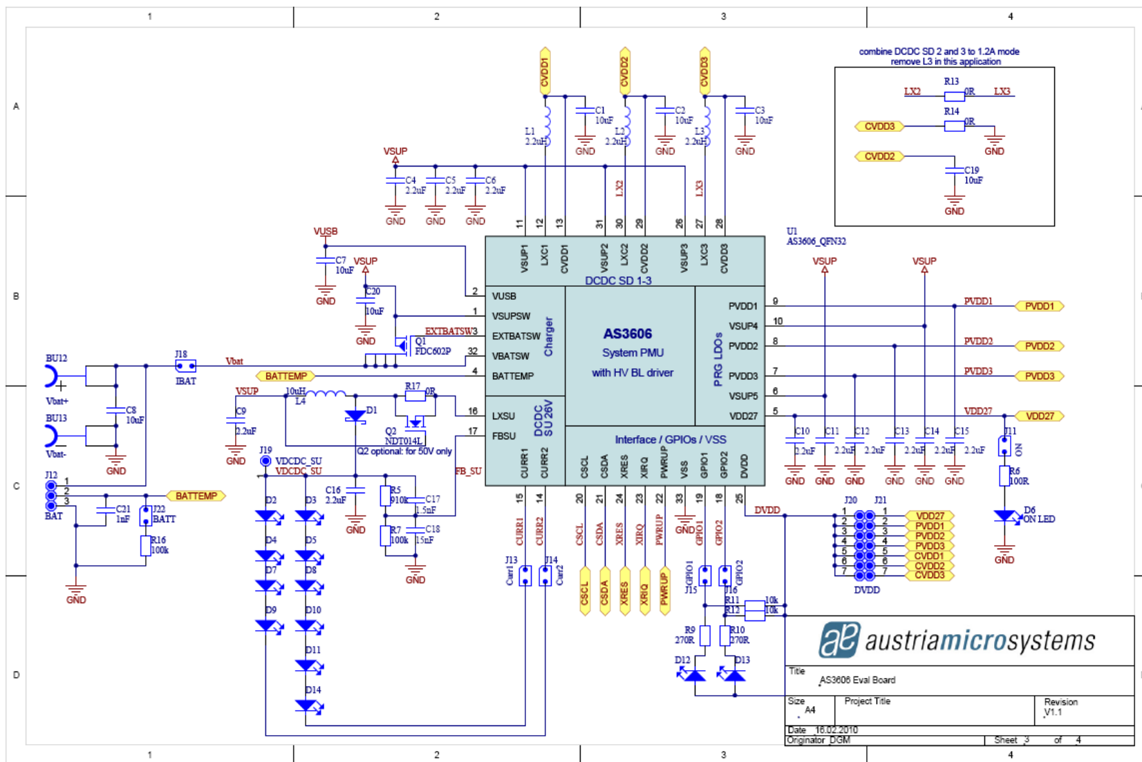
Application Schematic AS3606 Evalboard 1v1 – page1
